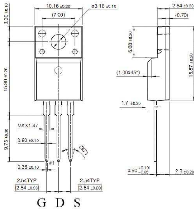
TO-220F
