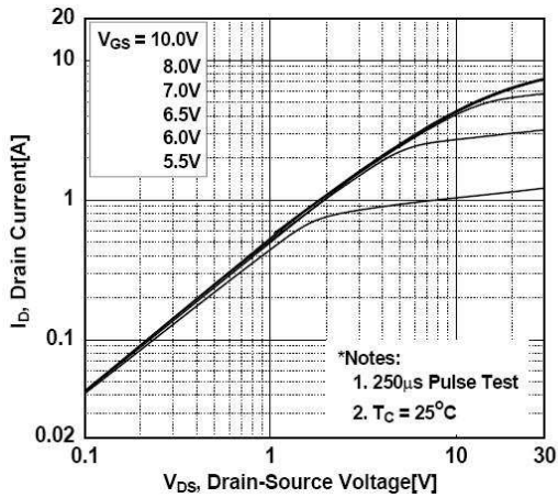
图1. 输出特性曲线 On-State Characteristics
