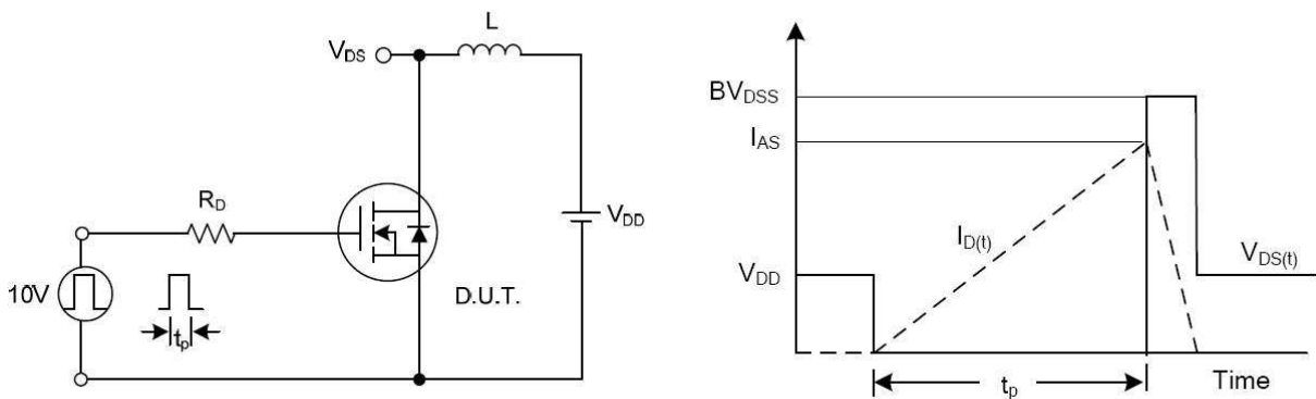
图12. 雪崩能量测试 Fig.12 Unclamped Inductive Switching Test Circuit & Waveforms
