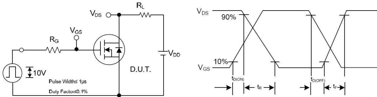
图11. 开关特性测试 Fig.11 Resistive Switching Test Circuit & Waveforms
