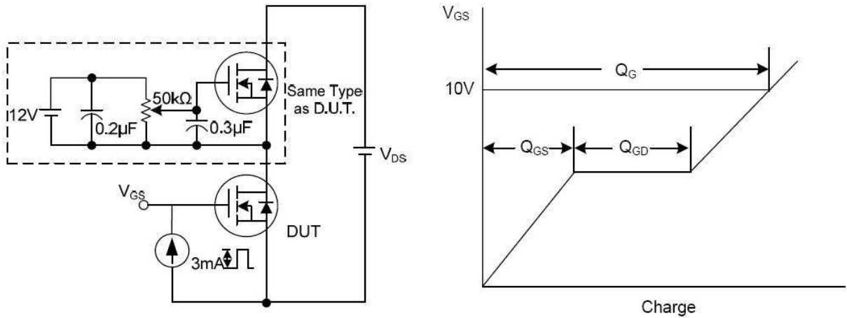
图11. 栅电荷测试 Fig.11 Gate Charge Test Circuit & Waveform
