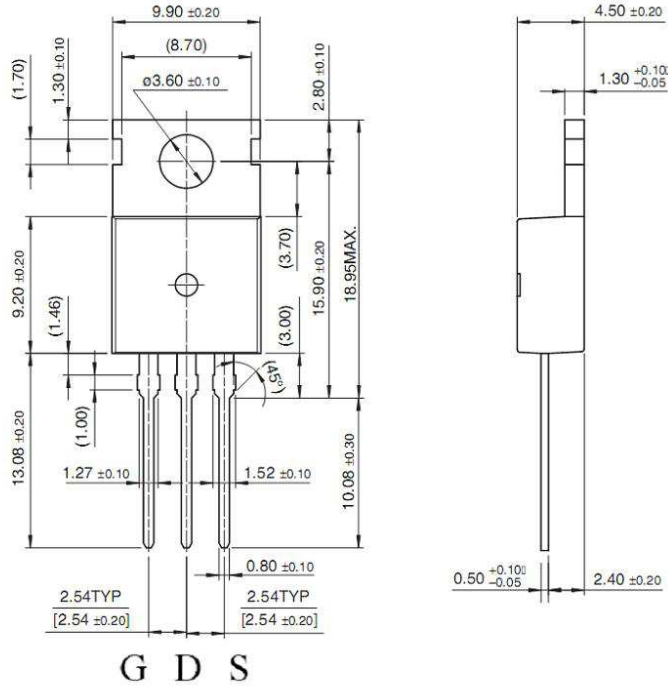
TO-220
