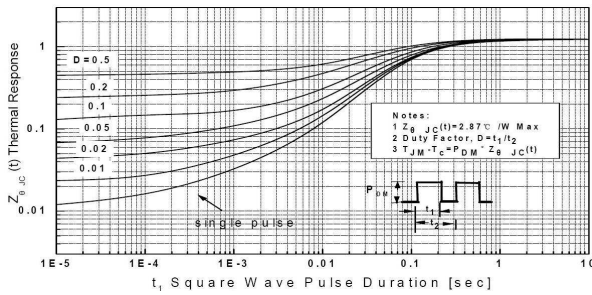
图9. 瞬态热响应曲线(TO-251/TO-252)
