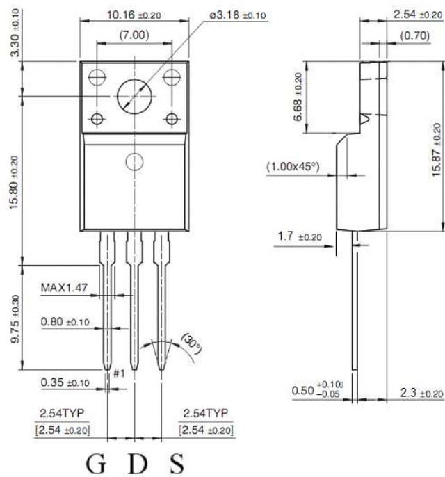
TO-220F
