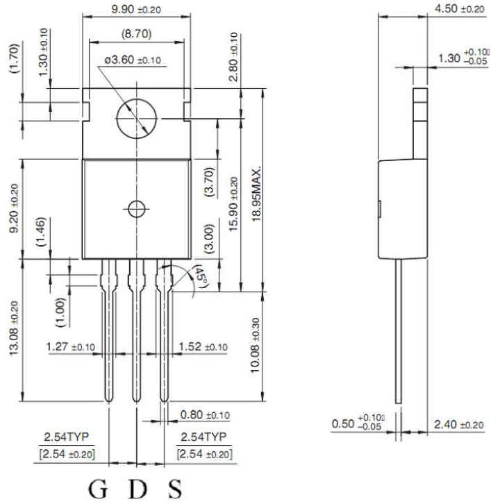
TO-220
